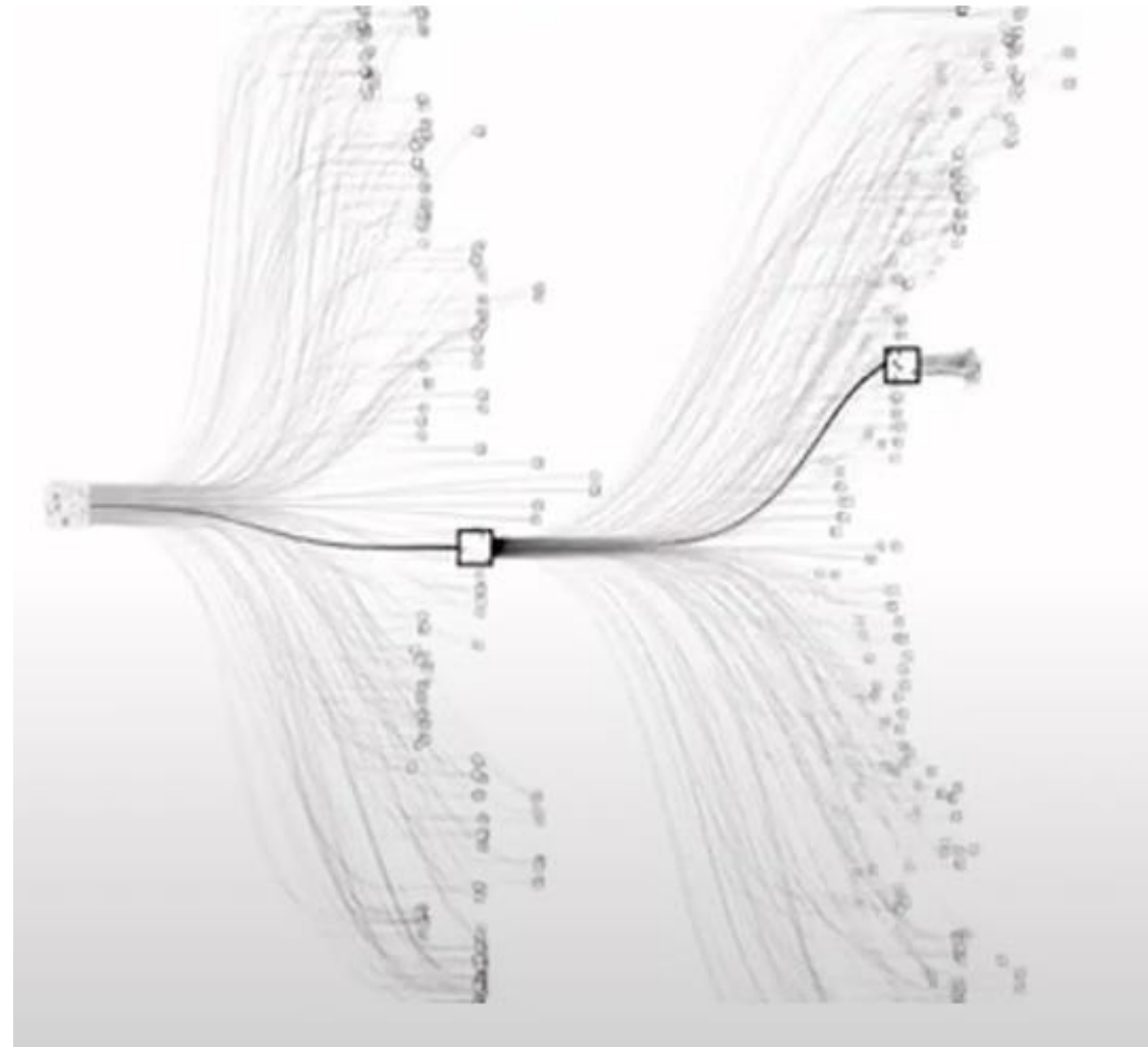
AlphaGo
