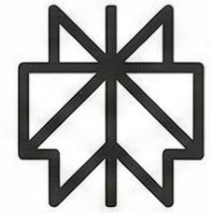
Perplexity
